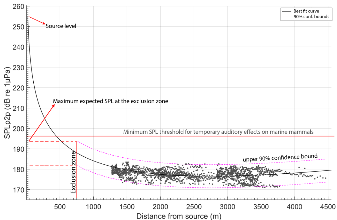
Fig. 4.6 The peak-to-peak SPL (SPLp2p) of each detected airgun impulse sound versus the absolute distance to the seismic source. The average and maximum expected SPL at the limits of the exclusion zone is compared to the minimum SPL threshold for temporary auditory effects on dolphins and physeters, as reviewed in Southall et al. (2019).
