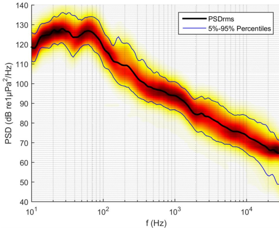
Fig. 4.4. Aggregated 10 sec PSDs concerning the full exclusion zone sound recording dataset.
