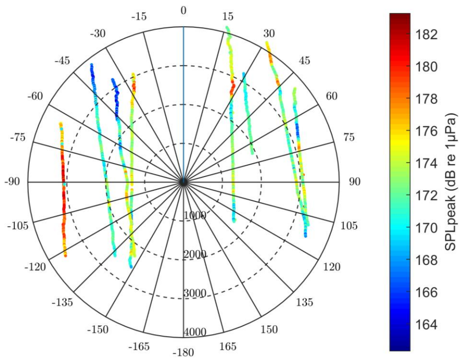
Fig. 4.5. Spatial distribution of estimated SPLpeak around the seismic source, integrated for each single T 5 -T 95 impulse sound duration.
