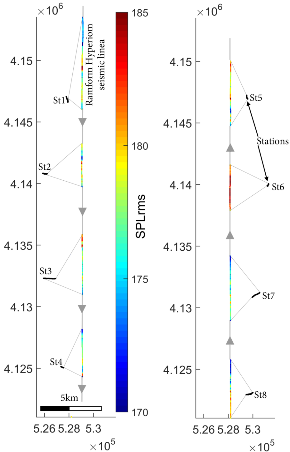
Fig. 2.2. The “Sea Master” stations and the relative seismic line of “Ramform Hyperion” that have been monitored for seismic impulse noise on December 21 st , 22 nd and 27 th 2022. Here SPLrms is illustrated and georeferenced in regard to both the seismic survey line and the monitoring stations. *Coordinates in UTM 34N.
