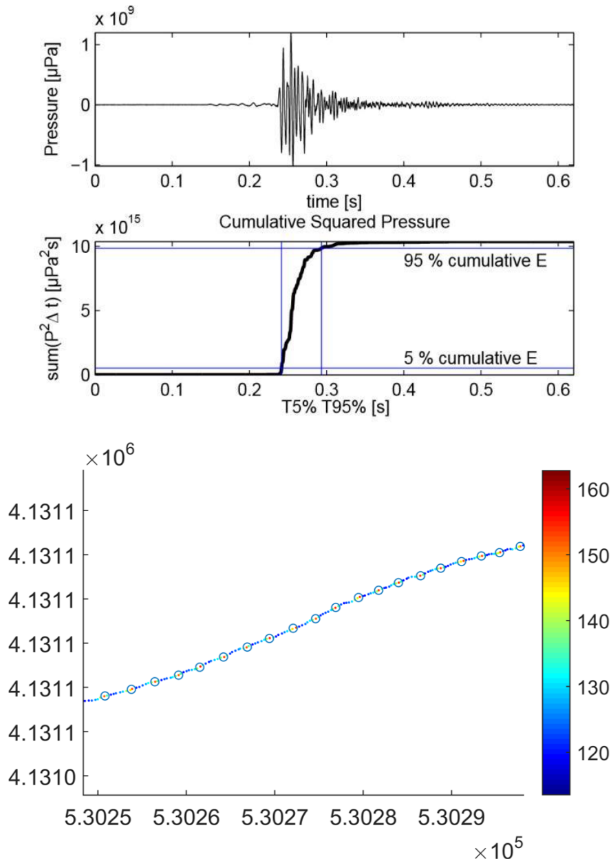
Fig. 3.1. Estimation of the 5% - 95% energy time intervals for an Airgun impulse sound through the cumulative squared pressure of the raw signal ( top figure ). SPLrms recorded on the monitoring line (colored dots) and detected impulses (circles). Colorbar corresponds to SPLrms dB re 1 μPa ( bottom figure ).
